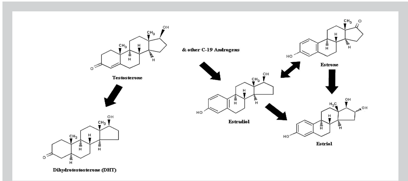
Figure 2. Basic synthesis of dihydrotestosterone and the estrogens: estradiol, estrone, and estriol.
