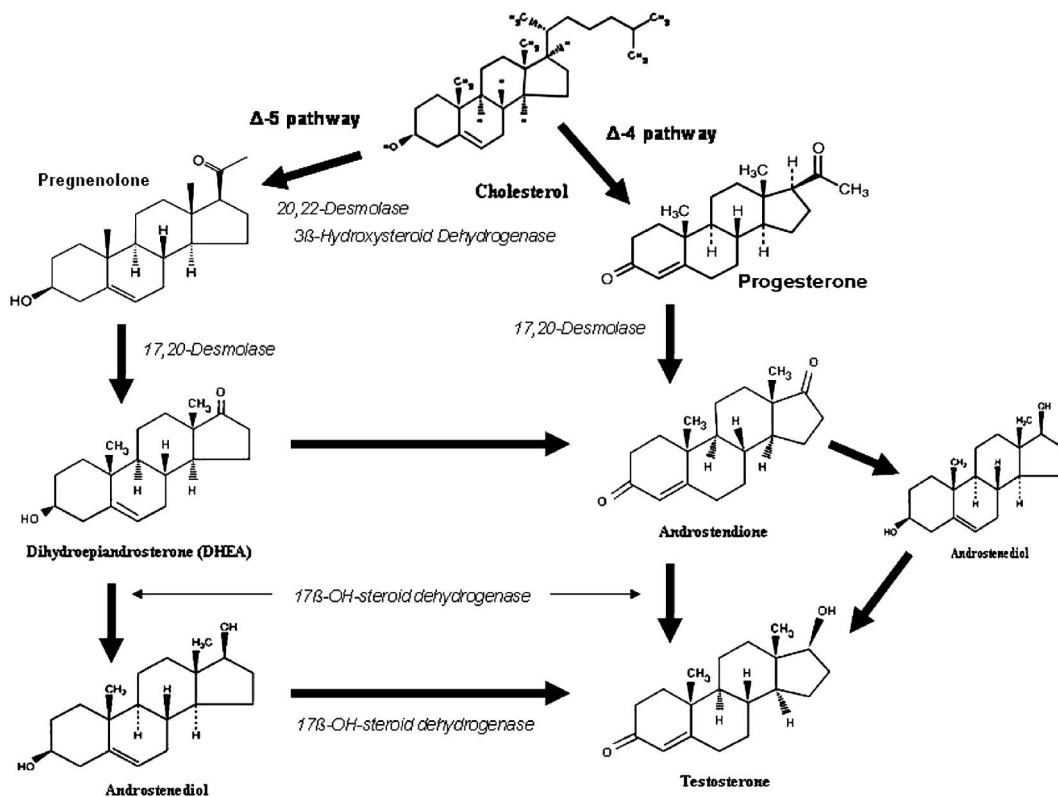
Figure 1. Testosterone synthesis.
